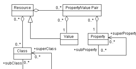
Figure 1: A UML conformant, modified version of the DCMI resource model.
