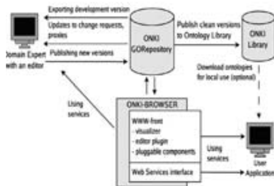
Figure 1: ONKI development and publishing process
