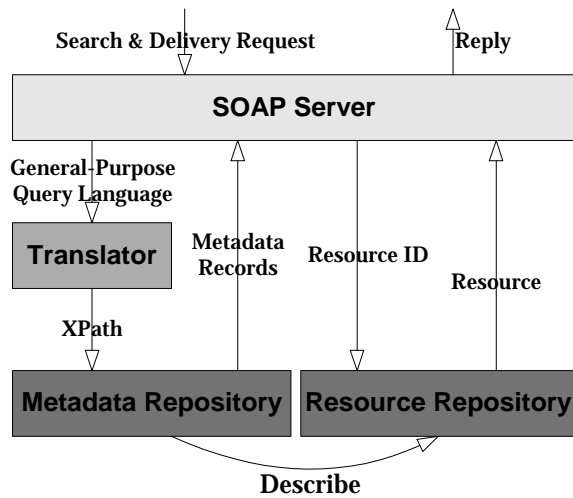
Figure 2. The Process of Handling Search & Delivery Requests in a Repository with a Native XML Database.
