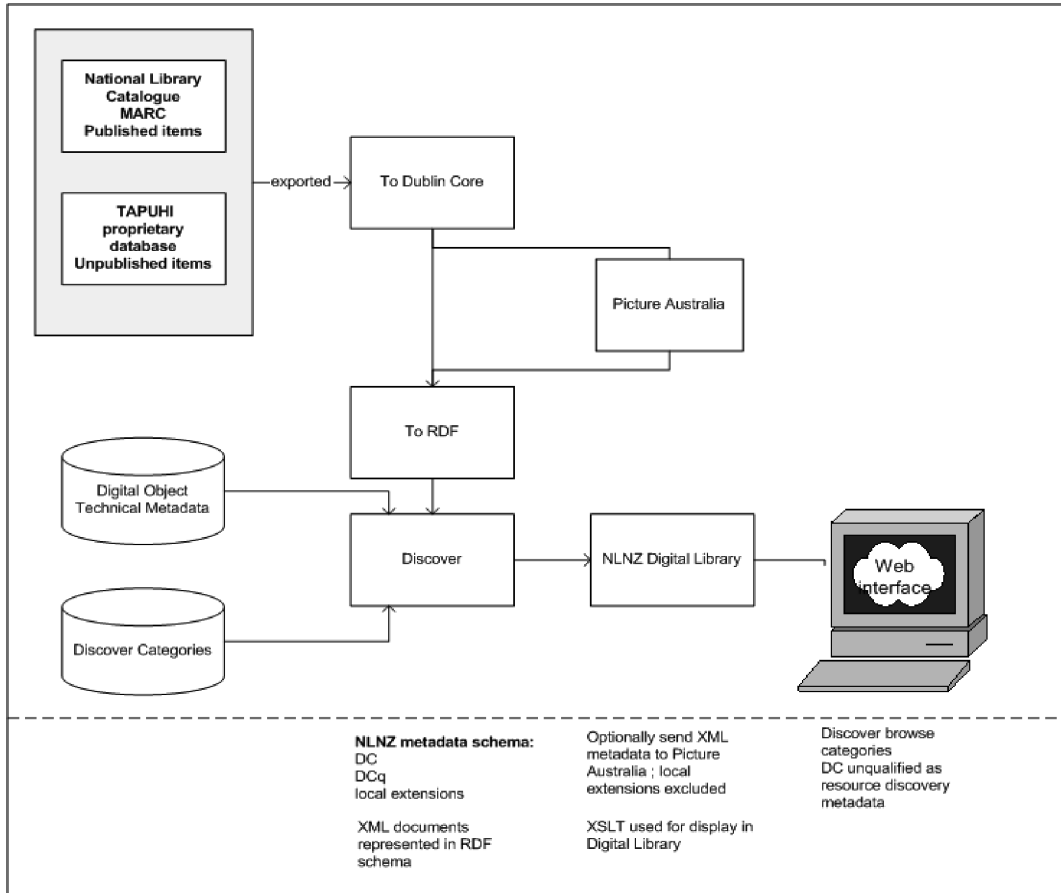
Figure 1. Discover overview
