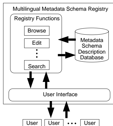
Figure 3. System Architecture of the Metadata Schema Registry
