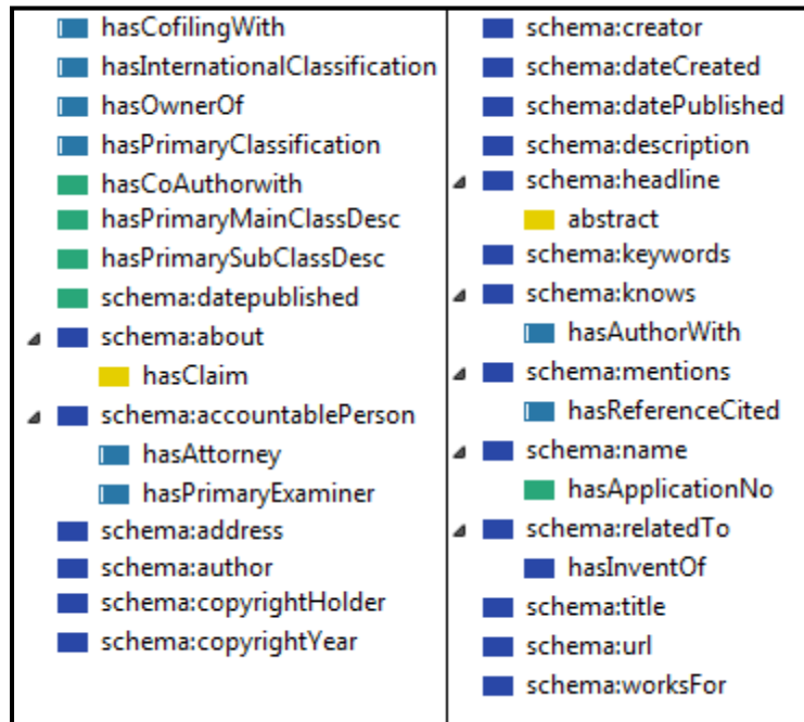
FIG.2. Overview of the Properties in Patent Ontology
